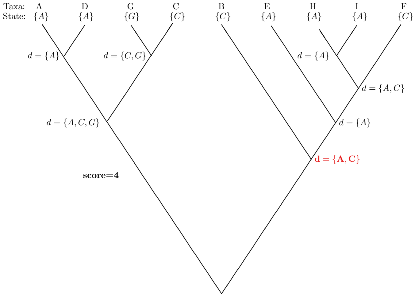
Figure 10: Fitch algorithm step 3 (sixth ancestral node) for that DNA sequence character shown in Table 8
