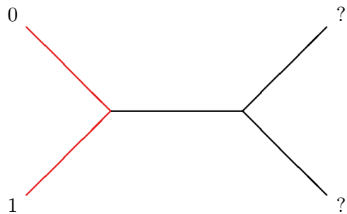
Figure 2: A character that could be explained by one change on one of two branches.
